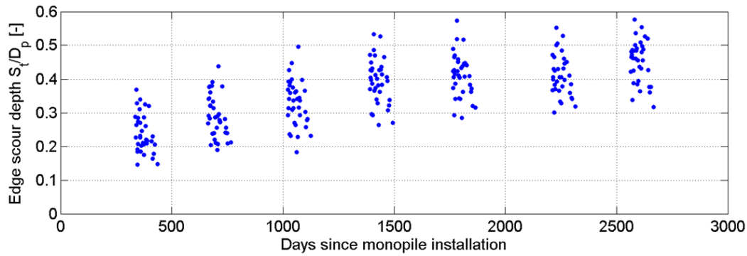
Figure 3.33. Maximum edge scour depth at downstream side for all 36 monopiles. Courtesy of Nordzeewind, a 50/50 joint venture of Shell and NUON.
