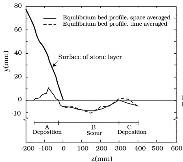
Figure A.9. Mean bed profile, space- and time averaged in cross-flow direction. Sketch of scour deposition pattern. Live-bed ( \theta > \theta_{cr} ). Test 1. Vertical scale is grossly exaggerated.
