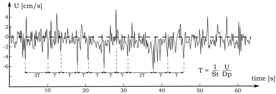
Figure 3.14. Time series of the stream wise velocity u measured at (x, y, z) = (2D_p, 0.5D_p, 0) ie. a measurement point in CFV-plane 2D_p downstream in correspondence with Fig. 3.8a and Fig. 3.12.
